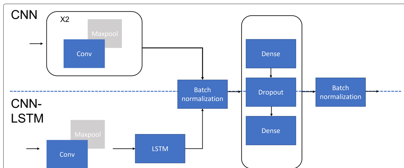
Fig. 4 Architectures of neural networks used in this study. The CNN is made of two convolution stacks (convolution layer + maxpooling). A filter size of five is used in the first convolution stack to serve as a motif detector. Thereafter, we used a larger filter size (32) in the next convolutional layer to capture larger patterns in the sequence. Following the convolution stacks, the features are flattened and batch normalized before passing through two dense layers using the ReLu activation function which are connected by a drop out layer. Finally, the output from the dense layer is passed to an output layer with a sigmoid activation to produce a final prediction value. Similar to the CNN model, we first used a convolution layer with a filter size of five to serve as a local motif detector for our CNN-LSTM model. After maxpooling, the output matrix is passed to an LSTM with 32 cells. Thereafter, the output from the LSTM is batch normalized and passed through two fully connected layers with the same configuration as our CNN model
